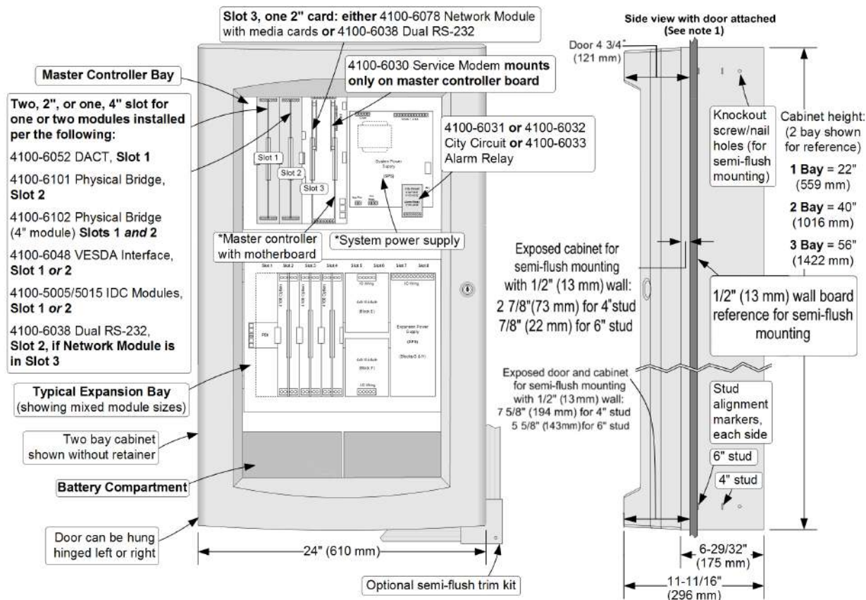
Figure 5: Mounting and CPU Bay Module Reference
